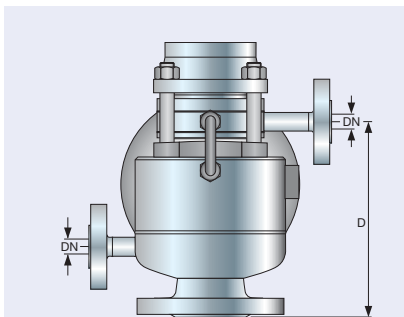
1. Heating connection with flange for balanced bellows construction
