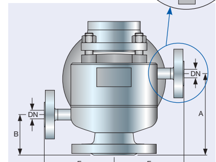
3. Heating connection with flange
